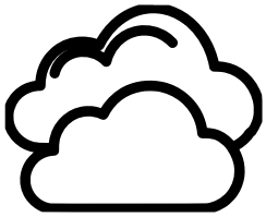
cloud
