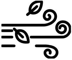
wind
